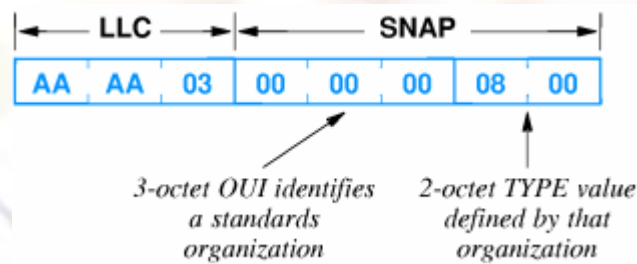
Figure 10.3. SNAP/LLC format
