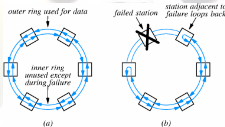
FIGURE 8.3 FDDI AND RELIABILITY:
