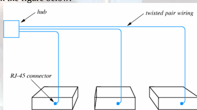
FIGURE 7.2 STAR NETWORK IN PRACTICE
