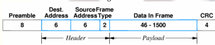
Figure 10.1 the Ethernet frame format
